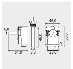
3/8" M. Contact 16 A - 380 V (AC1)
