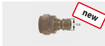
Plug : F. Hardened stainless steel. Max. 350 bar / 100 °C
