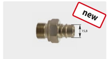
Plug : M. Hardened stainless steel. Max. 350 bar / 100 °C
