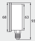
Ø 63 mm. 1/4" M. Housing stainless steel. Inlet at the bottom
