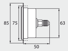
Ø 63 mm. 1/4" M. With mounting ring. Housing stainless steel. Inlet at the back
