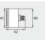
Ø 40 mm. 1/8" M. Housing plastic. Inlet at the back
