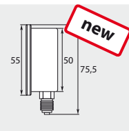
Ø 50 mm. 1/4" M. Housing stainless steel. Inlet at the bottom. Type WIKA
