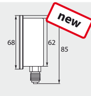
Ø 63 mm. 1/4" M. Housing stainless steel. Inlet at the bottom. Type WIKA
