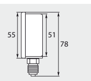
Ø 50 mm. 1/4" M. Housing stainless steel. Inlet at the bottom
