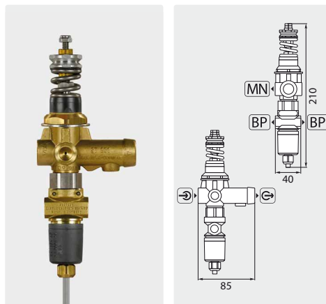
ST-261 for panel mounting with pressure switch
