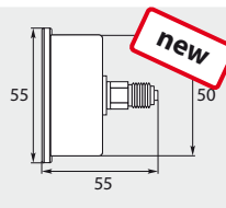
Ø 50 mm. 1/4" M. Housing stainless steel. Inlet at the back. Type WIKA
